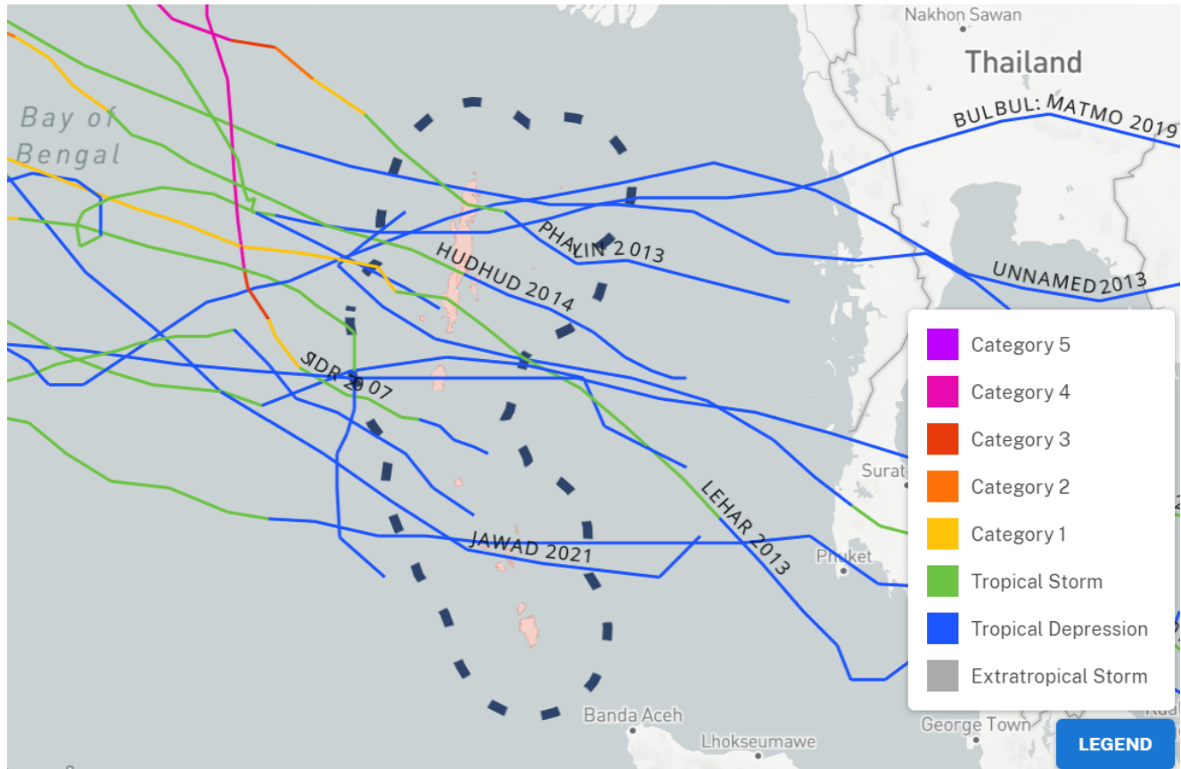
Figure 10: Cyclone tracks in the last 20 years
